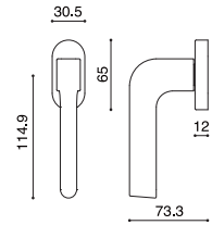
Window Handle 209W-O
