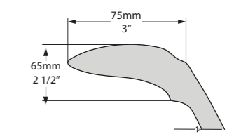
Rim Detail
