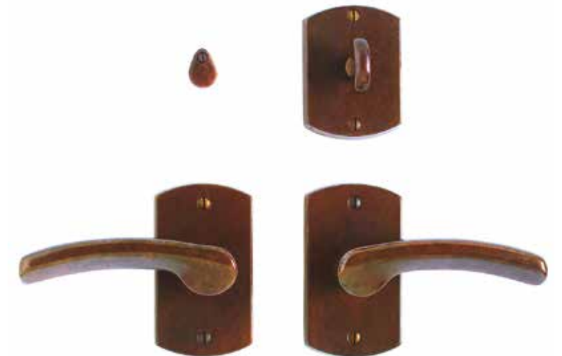
ESCUTCHEON 2 1/2" x 4 1/2" FUNCTION PRIVACY MORTISE BOLT/SPRING LATCH LEVER L224 RIDGE PATINA SILICON BRONZE RUST PART # E504/E504 WITH IP512
