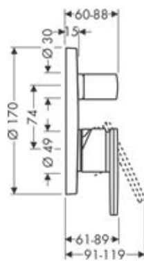
Single lever manual bath mixer for concealed installation with lever handle and integrated backflow prevention
