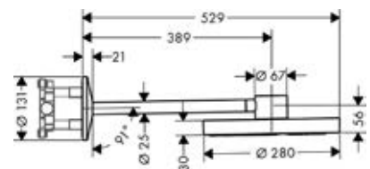
Overhead shower 75 1jet EcoSmart with shower arm
