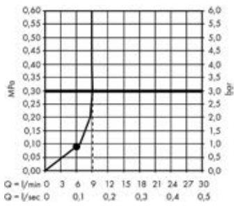
Hand shower 75 1jet EcoSmart # 48651820
