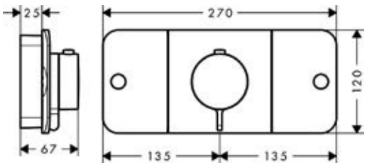
Thermostatic module for concealed installation for 2 outlets
