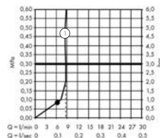
Overhead shower 75 1jet EcoSmart with shower arm # 48490820
