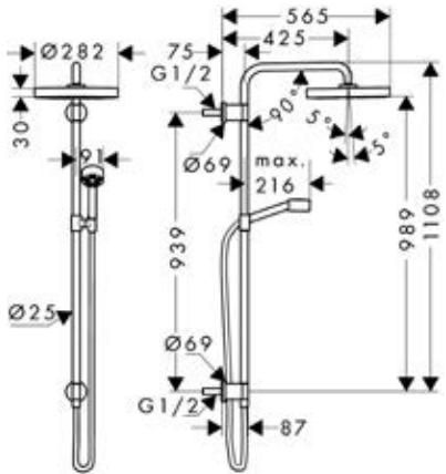
Showerpipe 280 1jet for concealed installation
