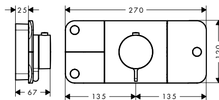
Axor One Thermostatic module for concealed installation for 3 functions
